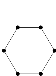
(a) 1D Simplicialkomplex
