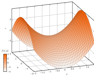
(b) S = V(X^2 - Y^2 - Z)
